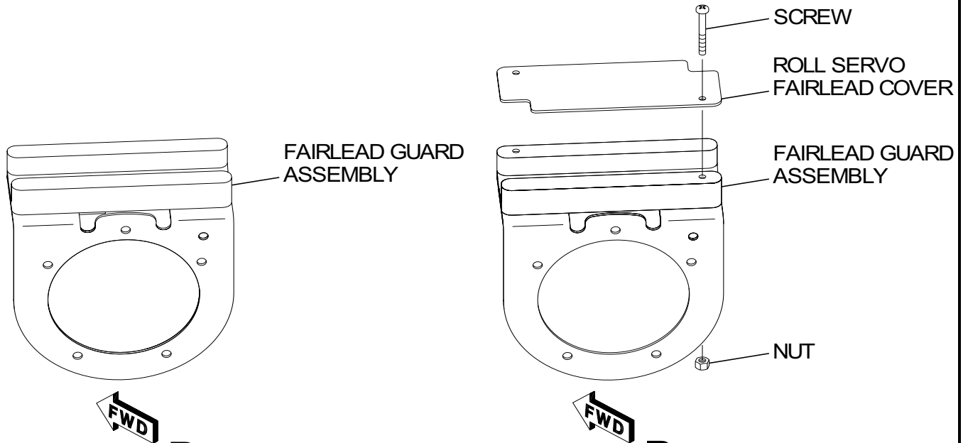
Figure 201 : Sheet 2 : Autopilot Roll Servo Installation
