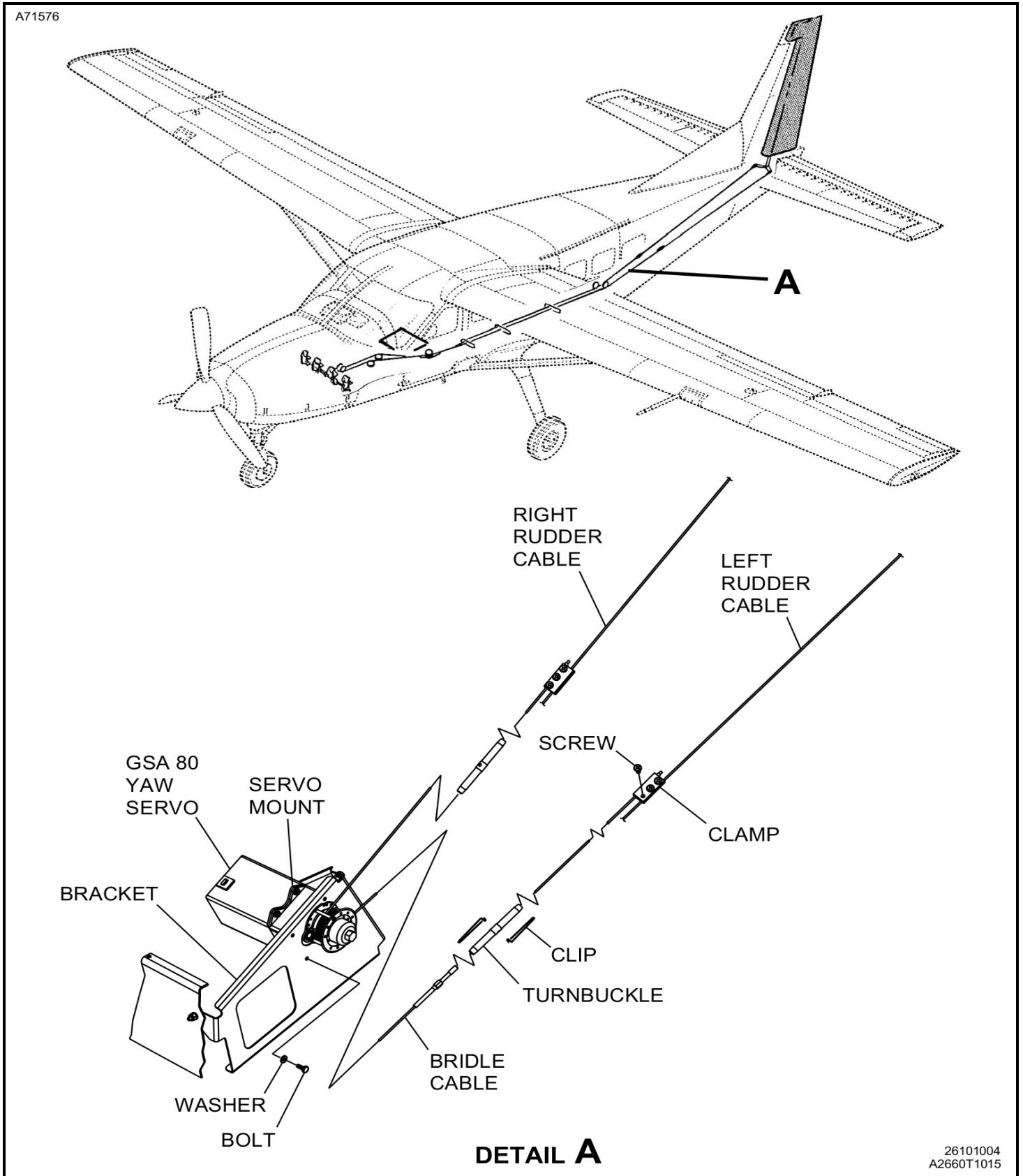
Figure 203 : Sheet 1 : Autopilot Yaw Servo Installation
